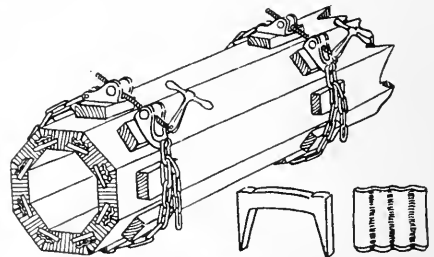
FIG. 423. CLAMPING MITERS.
